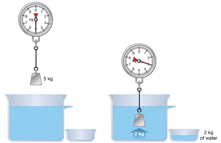
Archimedes' principle
